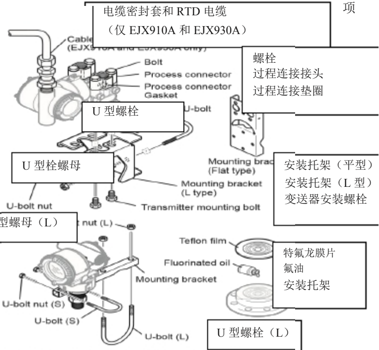
Figure 2.1 Transmitter Mounting Hardware
